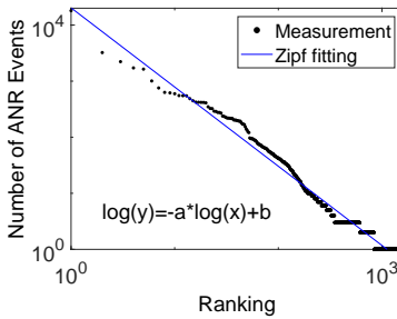
Figure 8: Ranking of apps by their number of ANR events. Here a = 1.41 and b = 4.31 .
