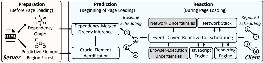
Fig. 1. Architectural overview of SipLoader, an SI-oriented web page loader that leverages the cumulative reactive scheduling framework.
